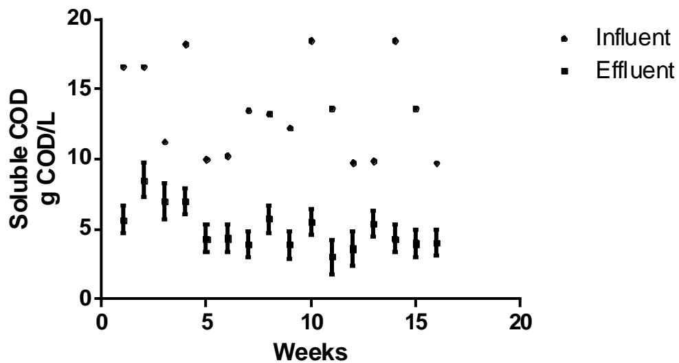
Figure C.8: Soluble COD influent and effluent concentrations for 16 weeks of Phase I
